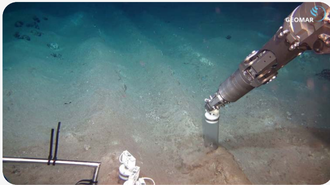
FIGURE 5: a 26-year-old test-mining track illustrates how slowly abyssal ecosystems of the deep seabed recover from physical disturbance. Image: sampling the DISCOL plow tracks. Image: Geomar, ROV Kiel 6000
